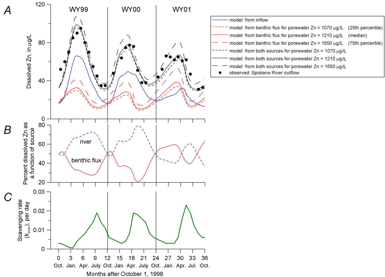
Figure 14.—Results of box model calculations for dissolved Zn in Lake Coeur d'Alene. A , Comparisons of measured and modeled dissolved Zn concentrations as a function of water years (WY) 1999 through 2001, taking into account variable discharge and dissolved Zn concentrations in the inflow and outflow and benthic fluxes. Concentrations of dissolved Zn as a function of time in the St. Joe and St. Maries Rivers were assumed to be constant at a value of 1.5 mg/L for the model runs. B , Relative contributions of dissolved Zn to the lake from inflowing rivers and from benthic flux. C , Model values for the scavenging rate coefficient ( k_{\text{scav}} ) that fit observed dissolved Zn concentrations in the outflow.
