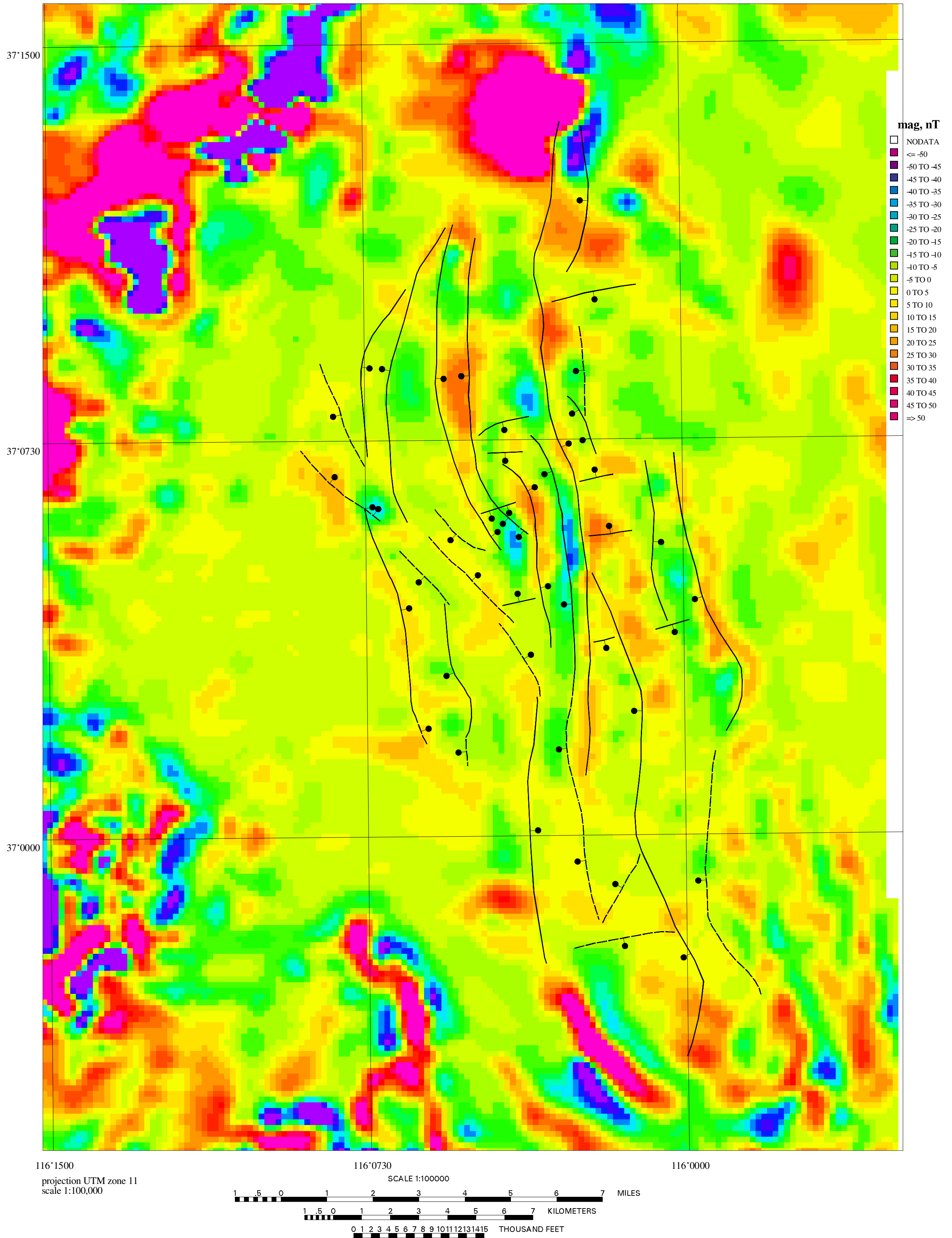
figure 5. Tertiary high-angle faults beneath Yucca Flat shown on magnetic anomaly surface Black lines, faults (dashed where less certain) with bar & ball on downthrown side
