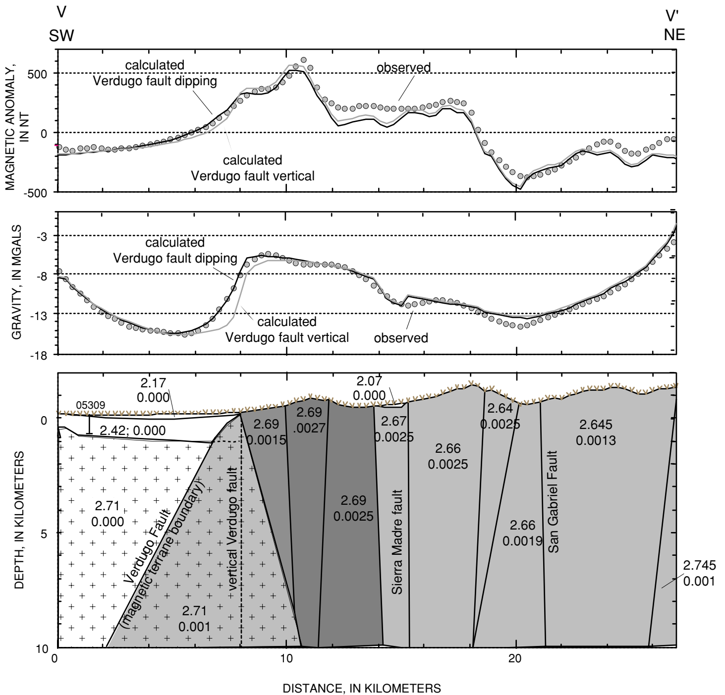
Figure 9a. Gravity and magnetic model across the Verdugo fault (profile V-V' on Figure 2). Numbers are densities in g/cm 3 and susceptibilities in cgs units. No vertical exaggeration. Sources extend to 10 km. The calculated gravity curve matches the observed gravity data if the Verdugo fault dips to the southwest. A dipping fault also matches the gentle decrease in magnetic values southwest of the fault better than if the Verdugo fault is vertical. Geometries of the San Gabriel and Sierra Madre faults are poorly constrained by the gravity data because of sparse gravity coverage along the profile (Fig. 4).
