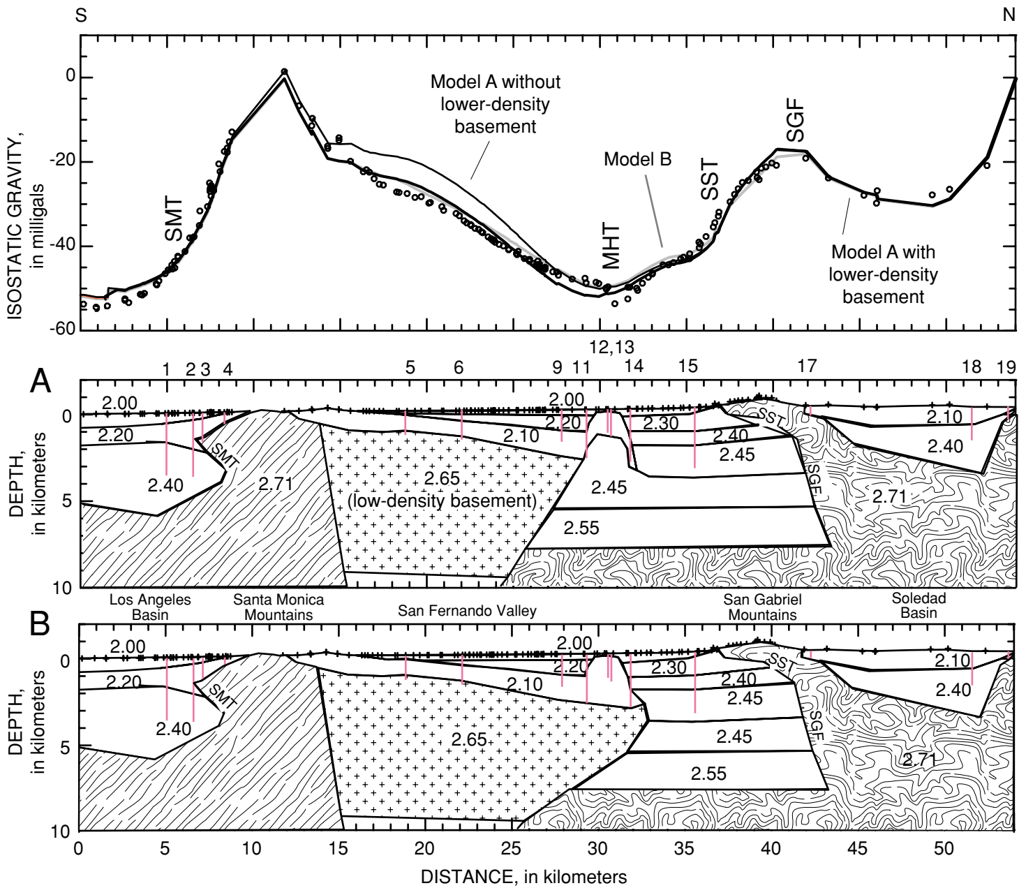
Figure 12. Gravity models across the San Fernando basin along profile A-A'. Small crosses on models are gravity station locations. Numbers in model are densities in \text{g}/\text{cm}^3 . Numbers above the model panel A refer to wells shown in Figure 1 and described in Table 1. MHT, Mission Hills thrust fault; SGF, San Gabriel fault; SMT, Santa Monica thrust fault; SST, Santa Susana thrust fault.
