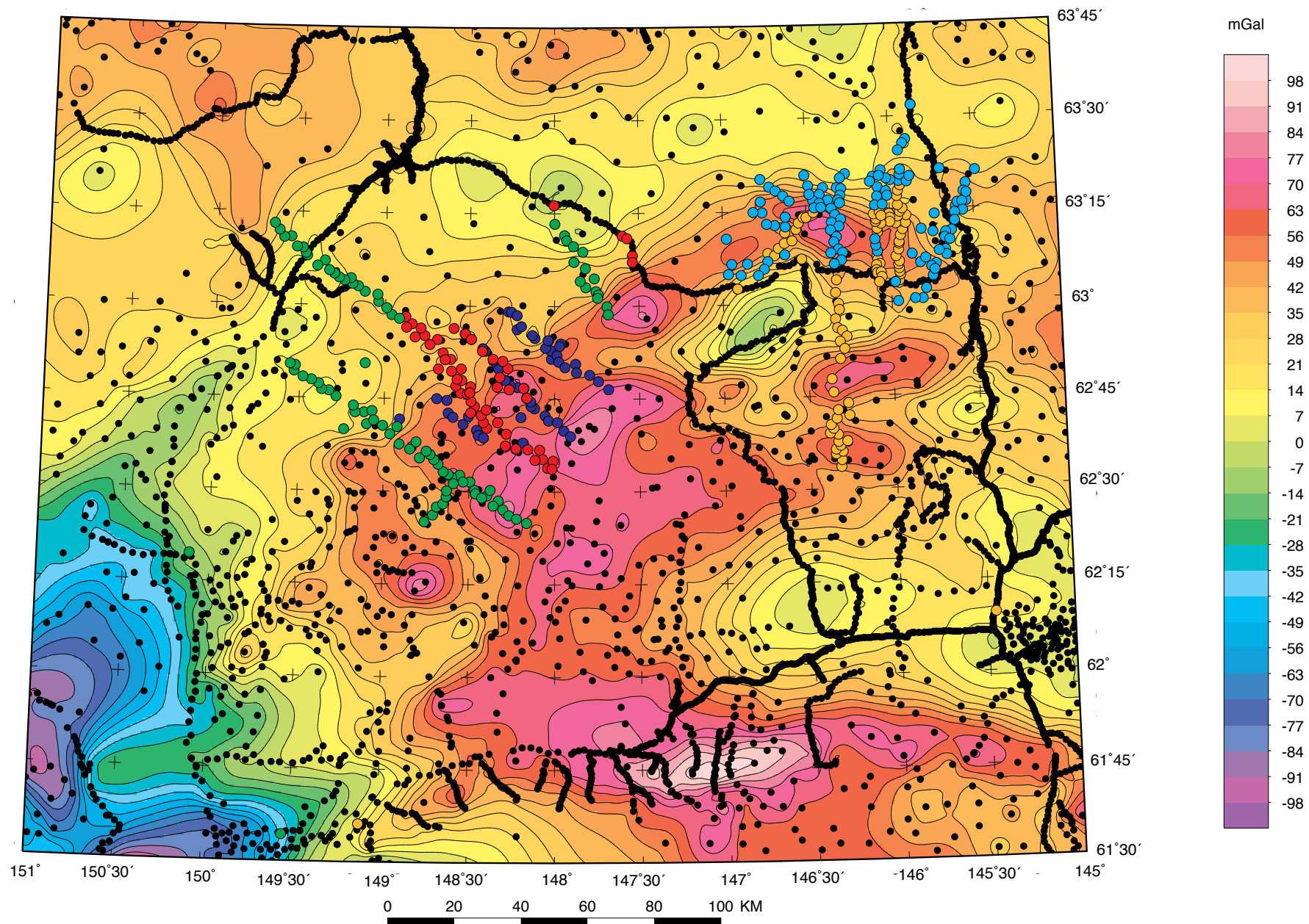
Figure 2. Isostatic gravity map of study area, contour interval 7 mGal. Data gridded at 1 x 1 km interval. Black circles, previous gravity stations; dark blue circles, 1999 data; red circles, 2000 data; green and orange circles, 2001 data; light blue circles, 2002 data.
